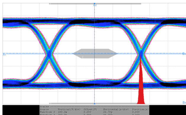
Figure 25. Eye at TP3 (Output of TMDS261) With 3-m, 28-AWG HDMI Cable, 3-Gbps Input TMDS Data Rate, Fastest Rise- and Fall-Time Setting on TMDS Outputs
