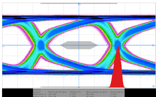
Figure 27. Eye at TP3 (Output of TMDS261) With 20-m, 24-AWG HDMI Cable, 2.25-Gbps Input TMDS Data Rate, Slowest Rise- and Fall-Time Setting on TMDS outputs
