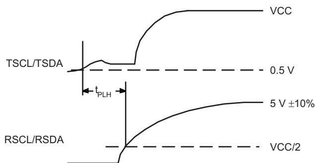
Figure 29. Waveform of Driver T Turning Off
