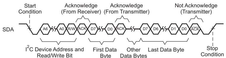
Figure 45. Multiple-Byte Read Transfer
