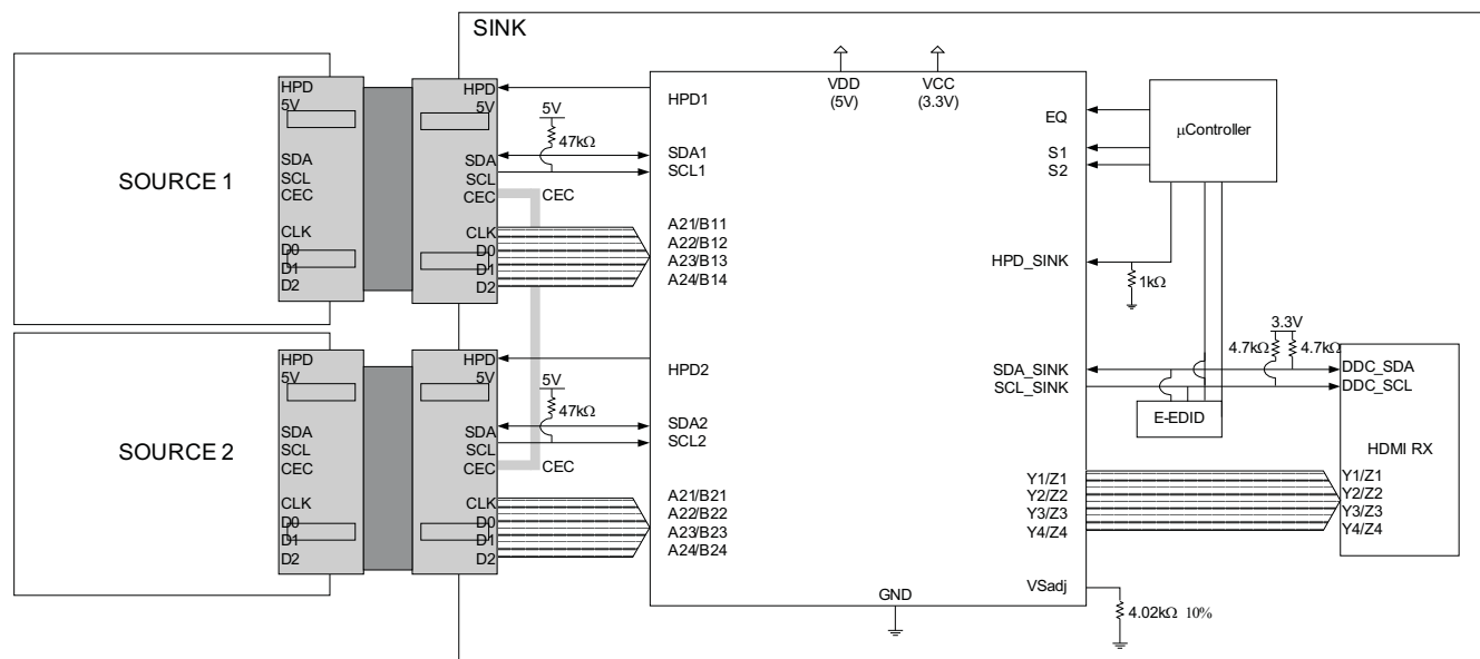
Figure 34. Two-Port HDMI-Enabled DTV With TMD5261 – CEC Commands Passing Through
